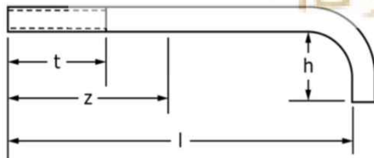
Anchor Bolt with Hook
