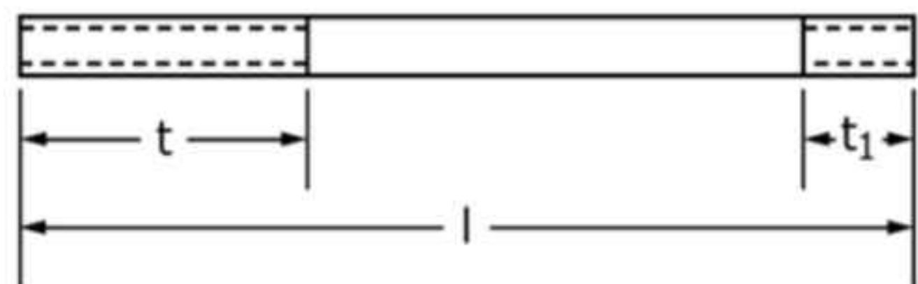
Straight Anchor Bolt
